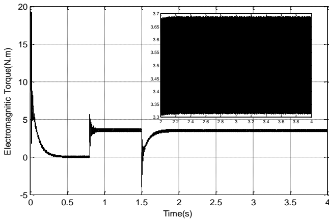
figure 3.c: Torque for healthy motor
