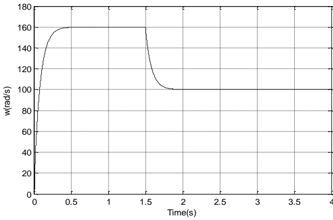
figure 3.a Speed response
