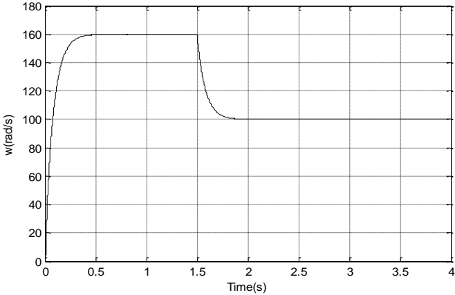
figure 4.a: Speed response
