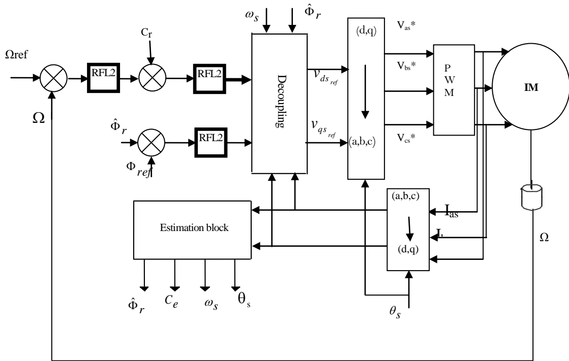
Figure 2: Speed control block by the direct method using regulator fuzzy type-2
