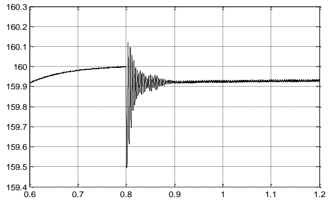
figure 3.b: Zoom of Speed
