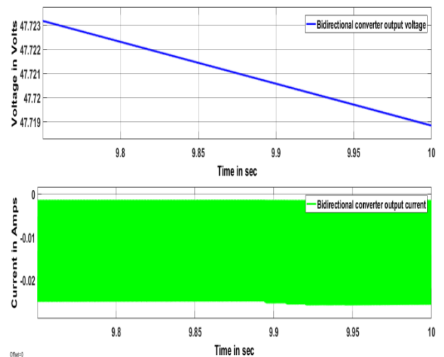
Figure 7(c). BDC output voltage and current
