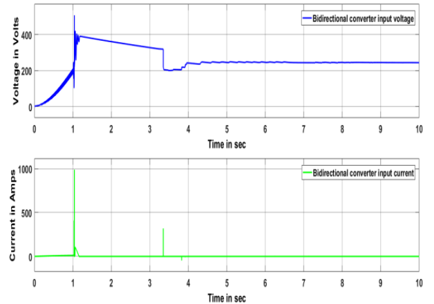
Figure 6(b). BDC input voltage and current
