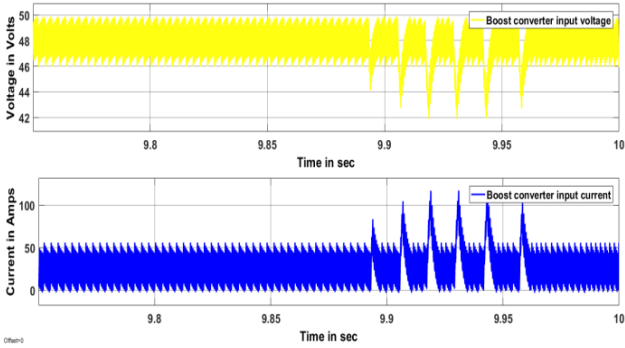
Figure 7(d). UDC input voltage and current
