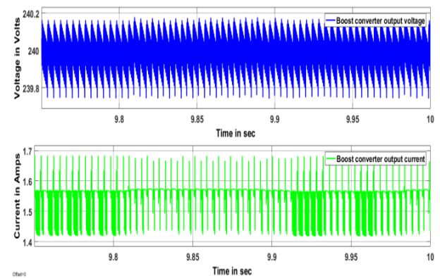
Figure 8(e). UDC output voltage and current
