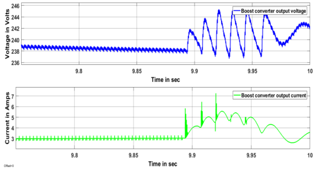
Figure 7(e). UDC output voltage and current
