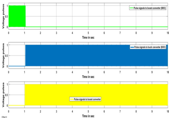
Figure 8(a). The pulse generated by the controller to UDC and BDC converters
