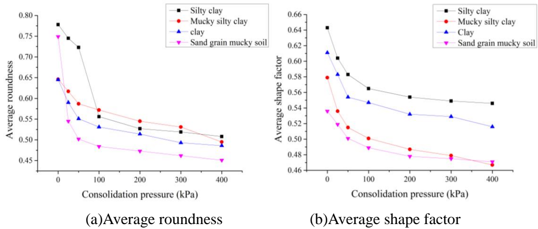
Fig. 7 Shape factors of four types of soil under different consolidation pressures
