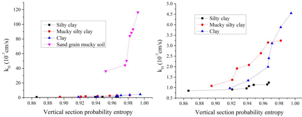
(a) Graph of curve k_H - H_m (b) Partial amplification graph of curve k_H - H_m
