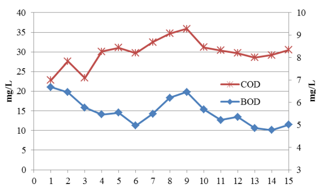
Fig.6. BOD 5 and COD value of the effluent
