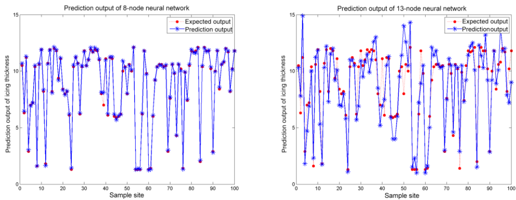
c) Prediction simulation curve of 8-node BP neural network
