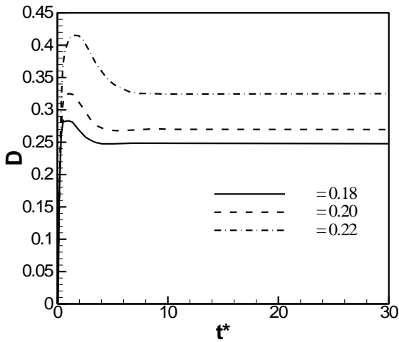
Figure 7. Bubble deformation versus dimensionless time at three different bubble sizes
