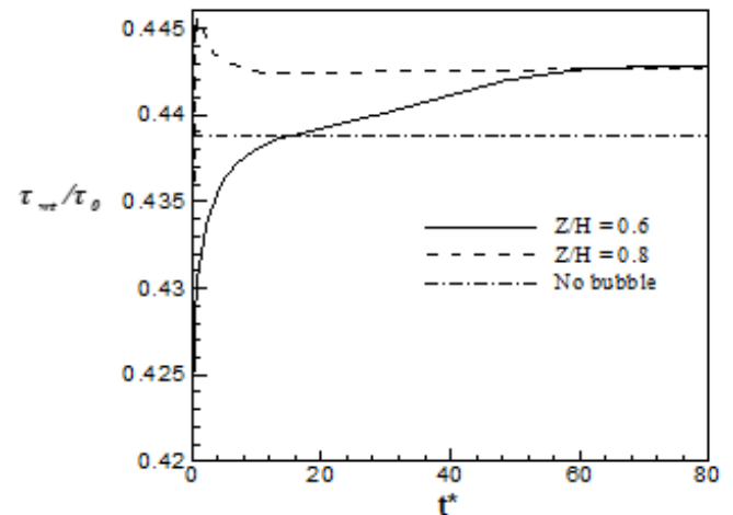
Figure 18. Impact of bubble's initial position on shear tension on the upper wall. Bubble has been released from the initial position of z_0/H = 0.6 and z_0/H = 0.8
