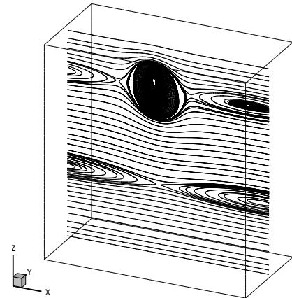
Figure 3. Streamlines in the middle section in the y -direction for a bubble with capillary number Ca = 0.3 .
