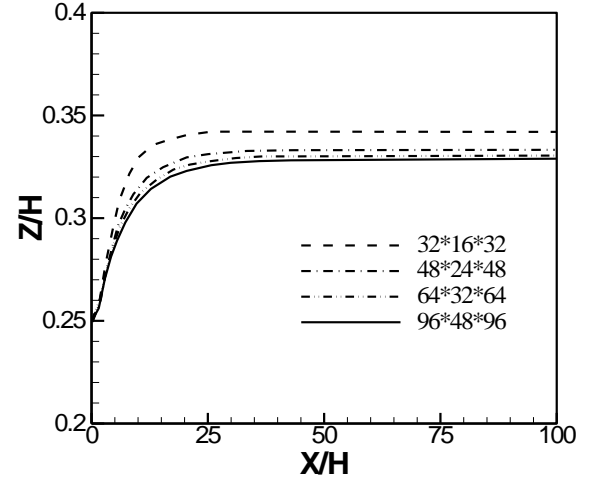
Figure 2. The lateral position versus the axial location of a bubble at four different grid resolutions.
