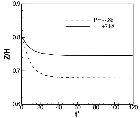
Figure 8. Effect of the pressure gradient on the lateral migration of a bubble
