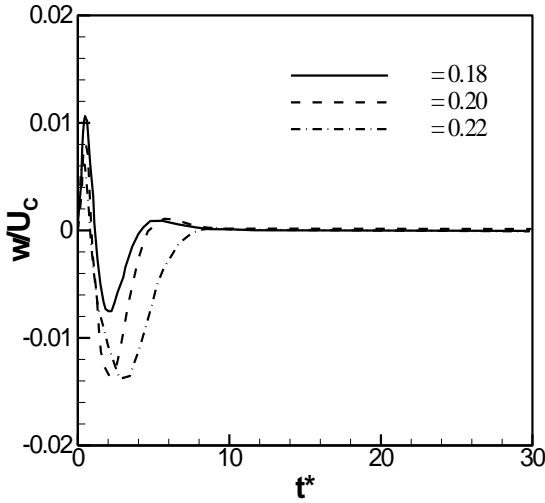
Figure 6. Lateral velocity versus dimensionless time at three different bubble sizes
