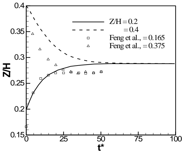
Figure 4. Comparison of the simulated Segre-Silberberg effect with the simulation of Feng et al. [19-20]
