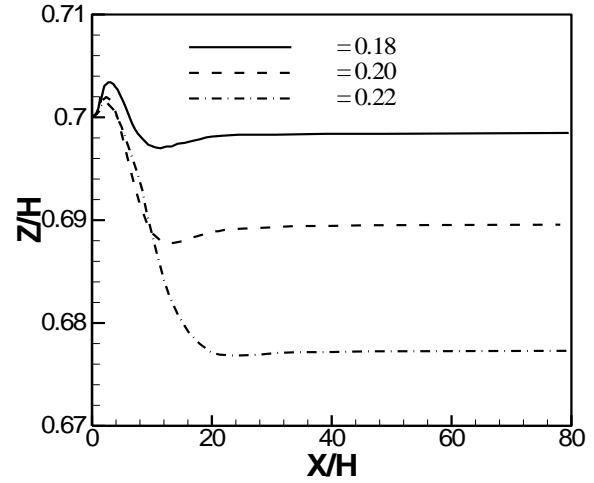
Figure 5. The lateral position versus the axial position at three different bubble sizes
