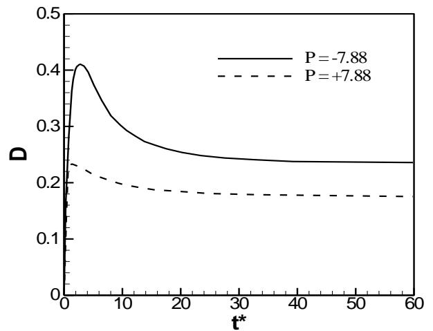
Figure 9. Effect of the pressure gradient on Taylor deformation
