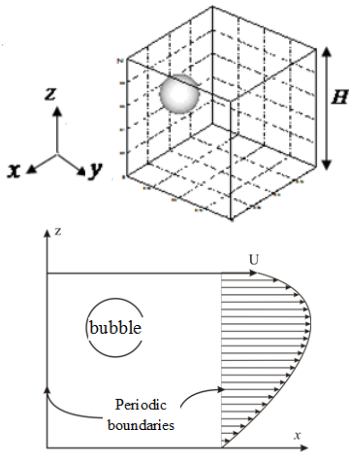
Figure 1. The geometry for the simulation of a bubble in a channel
