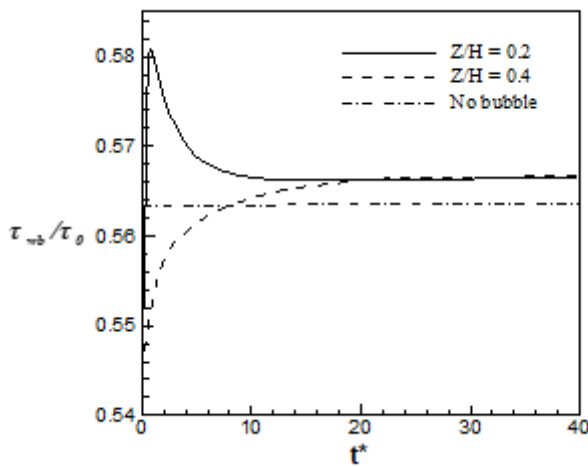
Figure 15. Initial position effect of a bubble on shear tension on the bottom wall. The bubble has been released from the initial position of z_0/H = 0.4 and z_0/H = 0.2
