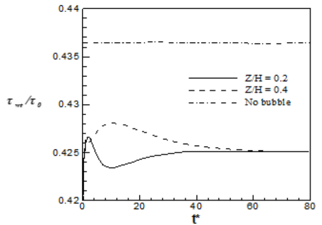
Figure 17. Impact of bubble's initial position on shear tension on the upper wall. Bubble has been released from the initial position of z_0/H = 0.2 and z_0/H = 0.4
