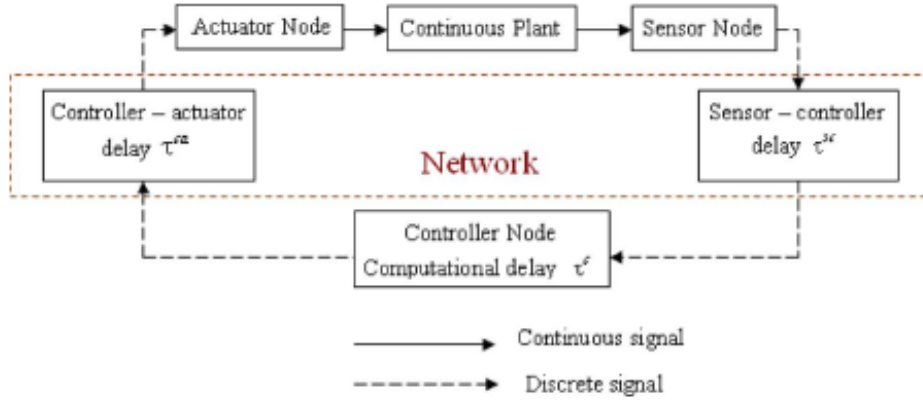
Fig.1 A typical networked control system
